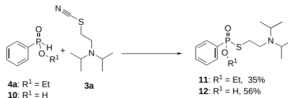
Scheme 4. Synthesis of VX analogues (THF, 70 °C, 24 h or neat, 25 °C, 10 d).
