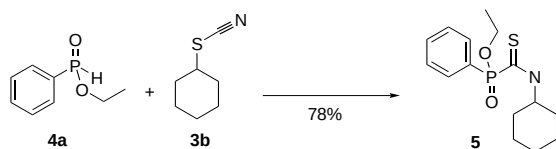
Scheme 2. Thermal Pudovik-like addition of cyclohexyl thiocyanate ( i\text{Pr}_2\text{NEt} , DMF, 110 °C).
