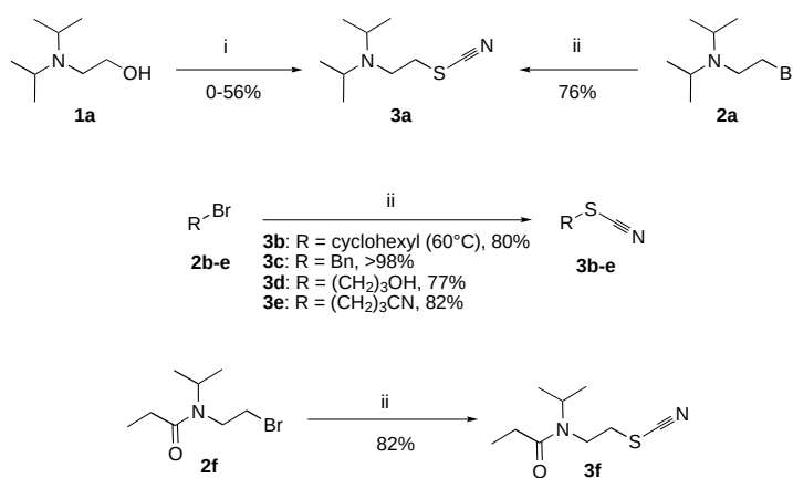
Scheme 1. Formation of thiocyanates: i) \text{Pb}(\text{SCN})_2 , \text{Br}_2 then \text{PPh}_3 , 0^\circ\text{C} , \text{CH}_3\text{CN} ; ii) \text{Me}_3\text{Si-N}=\text{C}=\text{S} , n\text{Bu}_4\text{NF} , THF.
