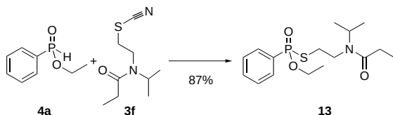
Scheme 5. Synthesis of phosphonothioate 13 (Phosphazene P 4 - t Bu (1%), toluene).
