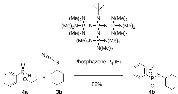
Scheme 3. Room temperature Pudovik-like addition of ethyl phenylphosphonate to cyclohexyl thiocyanate (phosphazene \text{P}_4\text{-}t\text{Bu} (1 %), toluene, 3 h, 25 °C).
